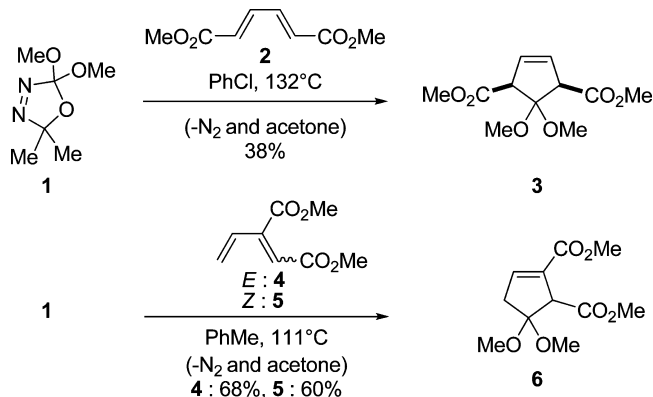
Scheme 1. Examples of Stereoselective Intermolecular (4 + 1)-Cycloadditions
