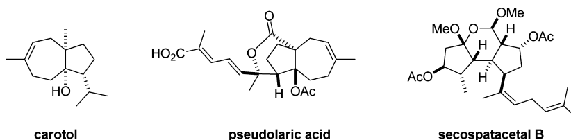
Figure 6. Three natural products that are targeted for synthesis.
