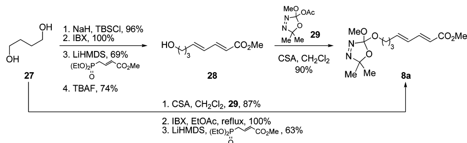
Scheme 4. Typical Preparation of a Cycloadduct Precursor
