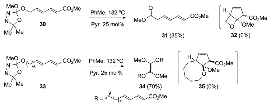
Scheme 5. Attempted Formation of Oxabicyclic Compounds 32 and 35
