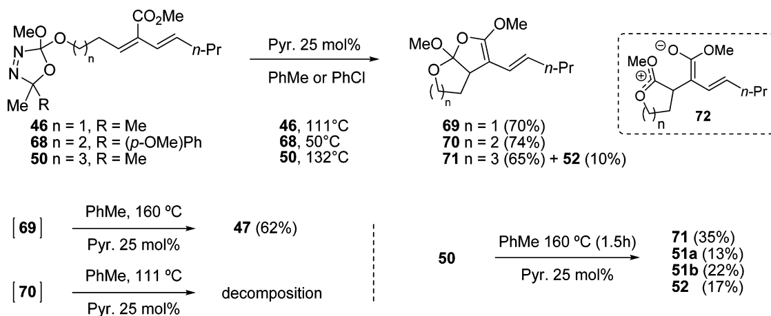
Scheme 17. Results from the Thermolysis of 46, 68, and 50
