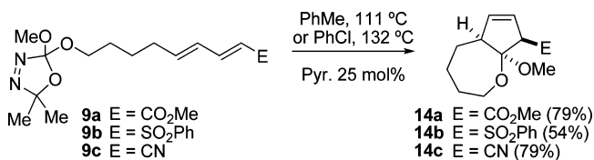
Scheme 6. Effect of the Nature of the Diene's Electron-Withdrawing Group on 7–5 Bicyclic Systems
