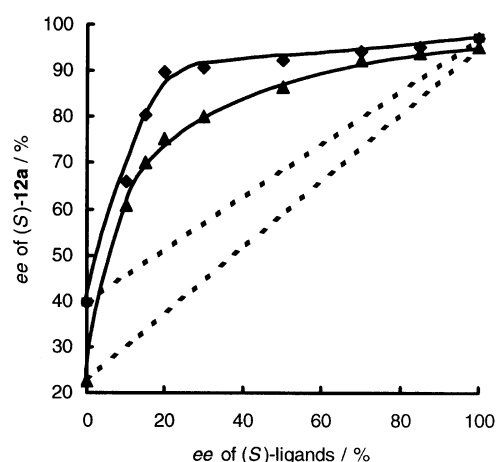
Figure 2. Comparison of nonlinear effects with dendritic (( S )- 10c , top line) and non-dendritic (( S )- 10a , bottom line) catalyst systems in the HDA reaction of 11 with 12a . The broken line indicates the expected ee values without a nonlinear effect.
