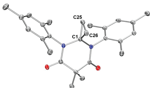
Figure 2. ORTEP diagram of 2a , with thermal ellipsoids drawn at 50% probability and H atoms omitted for clarity. Selected distances (Å) and angles (deg): C1–C25, 1.464(2); C1–C26, 1.471(2); C25–C26, 1.285(2); C25–C1–C26, 51.90(10); C26–C25–C1, 64.32(11); C25–C26–C1, 63.78(11).
