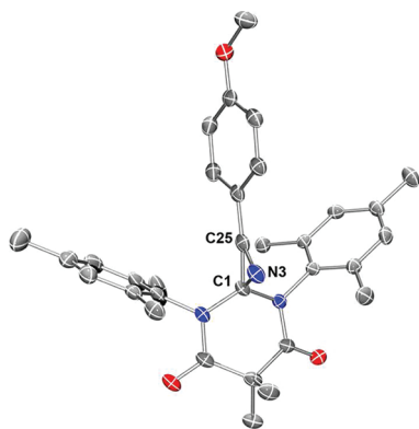
Figure 3. ORTEP diagram of 5c , with thermal ellipsoids drawn at 50% probability and H atoms omitted for clarity. Selected distances (Å) and angles (deg): C1–C25, 1.436(2); C1–N3, 1.5184(18); N3–C25, 1.2753(19); N3–C25–C1, 67.81(10); C25–N3–C1, 61.15(10); C25–C1–N3, 51.05(9).
