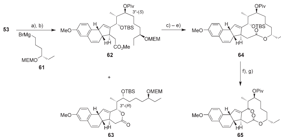
Scheme 11. Synthesis of the novel spinosyn analogue 65 : a) 1.15 equiv 61 , THF, −35°C, 1 h; b) 2×(5.0 equiv PivCl, 10 equiv NEt 3 , 1.0 equiv DMAP), CH 2 Cl 2 , reflux, 22 h, 62 : 42% (two steps), 63 : 29%; c) 4.0 equiv TMSI, 4.0 equiv NaI, MeCN, −35°C, 4.5 h; 81%; d) 10 equiv LiOH·H 2 O, THF/H 2 O 4:1, 40°C, 33 h; e) 4.0 equiv TCBzCl, 6.0 equiv NEt 3 , THF, RT, 1.5 h, then slow addition to 10 equiv DMAP, toluene, 75°C, 5.5 h, 74% (two steps); f) HF·pyridine/pyridine 1:3, 60°C, 14 h, 91%; g) 1.5 equiv DMP, CH 2 Cl 2 , RT, 20 min, 86%.
