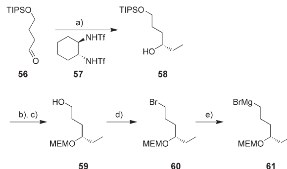
Scheme 10. Synthesis of C-6 fragment 60 : a) 10 mol % 57 , 2.0 equiv Ti(OiPr) 4 , toluene, 50°C, 30 min, then addition of 1.8 equiv ZnEt 2 at −65°C, 20 min, then addition of 56 at −20°C, 68 h, 96%, 98% ee ; b) 1.75 equiv MEMCl, 2.0 equiv DIPEA, CH 2 Cl 2 , RT, 5 h, 85%; c) 2.0 equiv TBAF·3H 2 O, THF, 0°C, 1 h, RT, 2 h, quant.; d) 1.5 equiv NBS, 1.2 equiv PPh 3 , THF, −15°C, 20 min, 85%; e) 5.0 equiv Mg turnings, 2 mol % Br 2 , THF, RT, 30 min, ≈50%.
