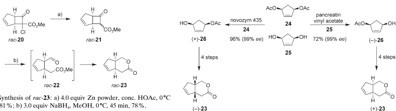
Scheme 5. Synthesis of (+)- 23 and (–)- 23 .
