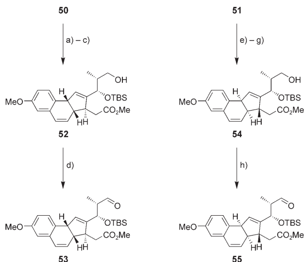
Scheme 9. Synthesis of aldehydes 53 and 55 : 53 : a) 4.0 equiv TBSOTf, 8.0 equiv DMAP, CH 2 Cl 2 , RT, 18 h, 90%; b) 25 equiv LiOH·H 2 O, THF/aqueous H 2 O 2 , −10°C, 10 d; c) 6.0 equiv N,N' -carbonyldiimidazole, THF, RT, 2.5 h, then addition of H 2 O and 9.0 equiv NaBH 4 , 0°C, 1 h, 53% [76% brsm] (two steps); d) 1.5 equiv DMP, CH 2 Cl 2 , 0°C, 3.5 h, 94%; 55 : e) 1.5 equiv TBSOTf, 2.0 equiv 2,6-lutidine, CH 2 Cl 2 , −10°C, 2.5 h, 85%; f) 25 equiv LiOH·H 2 O, THF/aqueous H 2 O 2 , −10°C, 6 d; g) 6.0 equiv N,N' -carbonyldiimidazole, THF, 0°C, 1 h, RT, 1.5 h, then addition of H 2 O and 6.5 equiv NaBH 4 , 0°C, 45 min, 72% (two steps); h) 1.5 equiv DMP, CH 2 Cl 2 , RT, 1.5 h, 90%.
