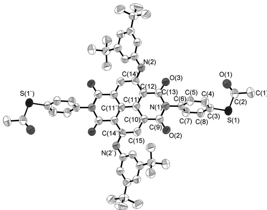
Fig. 1. X-Ray single-crystal structure of 1 (ORTEP representation, thermal ellipsoids set at the 40%-probability level). H-atoms have been omitted for clarity; only one orientation of the disordered 'Bu groups is shown. Selected bond lengths (in pm) and bond angles (in °): C(1)–C(2) 149.6(6), C(2)–O(1) 119.7(5), C(2)–S(1) 178.4(5), S(1)–C(3) 176.6(4), C(3)–C(4) 138.1(6), C(4)–C(5) 138.8(5), C(5)–C(6) 133.8(6), C(6)–C(7) 140.6(5), C(7)–C(8) 139.6(5), C(8)–C(3) 135.9(6), C(6)–N(1) 146.7(4), N(1)–C(9) 138.1(5), C(9)–O(2) 121.2(5), C(9)–C(10) 148.3(5), C(10)–C(11) 140.4(5), C(11)–C(12) 142.0(5), C(12)–C(13) 145.9(5), C(13)–O(3) 122.5(5), C(13)–N(1) 140.2(5), C(12)–C(14) 140.8(5), C(14)–N(2) 137.0(5), C(10)–C(15) 137.0(6), C(15)–C(14') 142.0(5), C(11)–C(11') 141.4(7); C(2)–S(1)–C(3) 102.7(2), C(9)–N(1)–C(13) 126.4(3).
