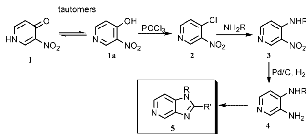
Scheme 1. General route to azabenzimidazoles ( 5 ) via 4-amino-3-nitropyridine ( 3 )
