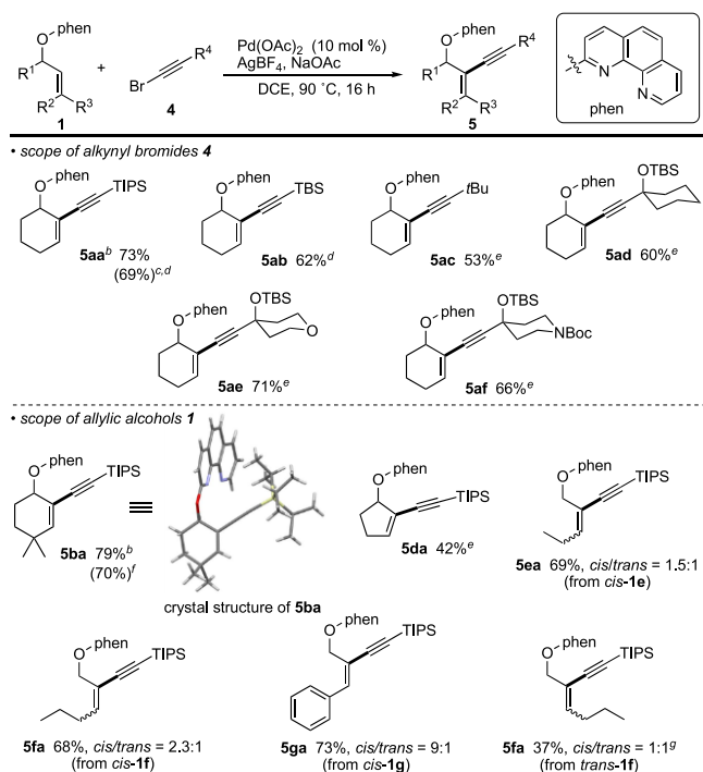
Scheme 3. Products of Phenanthroline-Directed, Pd-Catalyzed Regioselective C–H Alkynylation of Allylic Alcohols 1 with Alkynyl Bromides 4 a
