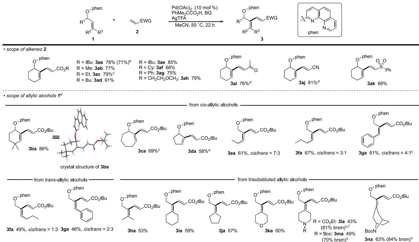
Scheme 2. Products of Phenanthroline-Directed, Pd-Catalyzed Regioselective C–H Alkenylation of Allylic Alcohols 1 with Electron-Deficient Alkenes 2 a
