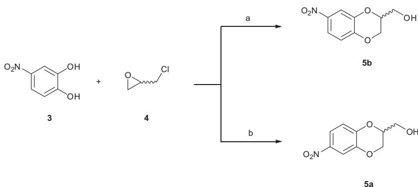
Scheme 1. Synthesis of the benzodioxine scaffold. Reagents and conditions: (a) \text{NaHCO}_3 , DMF, 80 ^\circ\text{C} , 12 h, (b) NaH, DMF, 80 ^\circ\text{C} , 12 h.
