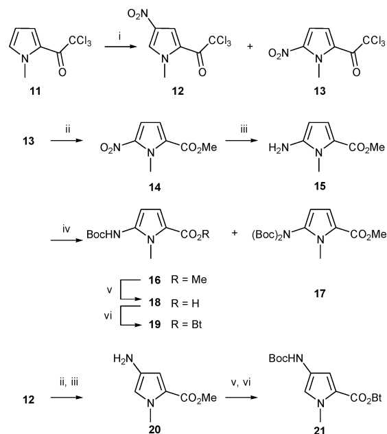
Scheme 1 Monomer synthesis. i) \text{HNO}_3 dropwise, \text{Ac}_2\text{O} , -40^\circ\text{C} –rt, (\text{CH}_3)_2\text{CHOH} , -40^\circ\text{C} ii) 0.05 equiv. DMAP, MeOH, rt, \text{N}_2 iii) \text{H}_2 (30 psi for 20 ), 10% Pd–C, THF (EtOAc for 20 ) iv) 1.2 equiv. \text{Boc}_2\text{O} , 1.1 equiv. TEA, 1,4-dioxane, \Delta v) 2 M aqueous NaOH, MeOH, 60^\circ\text{C} vi) HOBt, EDCI or DCC, DMF, rt, \text{N}_2 .
