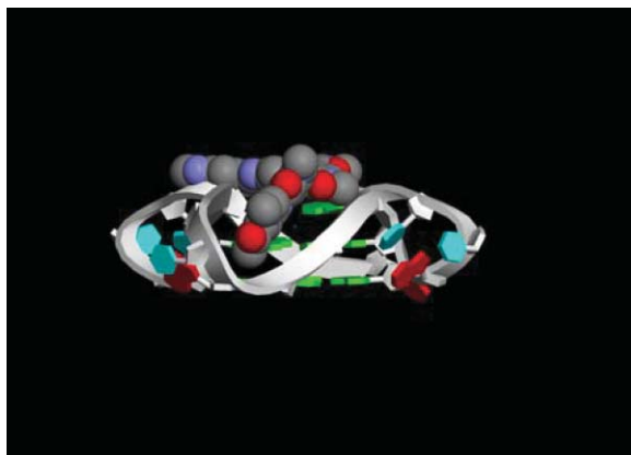
Fig. 2 A qualitative molecular model of a six-repeat pyrrole polyamide molecule (shown in space-filling mode), analogous to compound 5 , docked onto the crystal structure of the human 22-mer quadruplex structure 29 (with the bases and backbone shown in cartoon form). Two repeats of the polyamide are located in a quadruplex groove, and the others are stacked on a terminal G-quartet surface.
