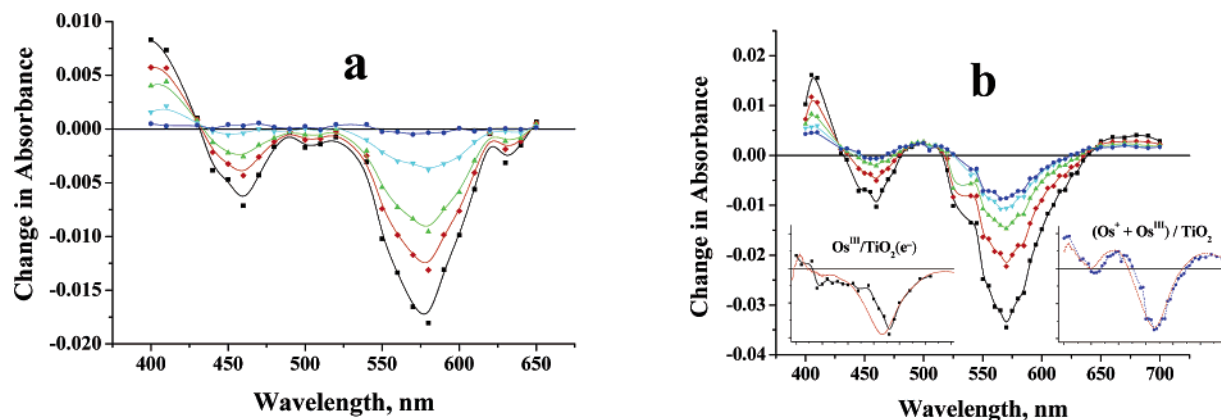
Figure 5. Transient absorbance spectra of (a) [\text{Os}(\text{bpy})_2(\text{dcbq})]/\text{ZrO}_2 and (b) [\text{Os}(\text{bpy})_2(\text{dcbq})]/\text{TiO}_2 following 417 nm light excitation ( 3.5 \text{ mJ}/\text{cm}^2 , 8 ns fwhm). The delay times for the \text{ZrO}_2 sample were as follows: 5 ns (black line, \blacksquare ), 10 ns (red line, \blacklozenge ), 15 ns (green line, \blacktriangle ), 30 ns (cyan line, \blacktriangledown ), and 100 ns (blue line, \bullet ). The delay times for the \text{TiO}_2 sample were as follows: 10 ns (black line, \blacksquare ), 25 ns (red line, \blacklozenge ), 100 ns (green line, \blacktriangle ), 500 ns (cyan line, \blacktriangledown ), and 2 \mu\text{s} (blue line, \bullet ). The inset shows a simulation over the same spectral range of the simulated spectra (dashed) overlaid with the experimental data obtained 5 \mu\text{s} after pulsed excitation of [\text{Os}(\text{bpy})_2(\text{dcbq})]/\text{TiO}_2 in 0.1 M \text{LiClO}_4 acetonitrile (left-hand side) and in neat acetonitrile (right-hand side).
