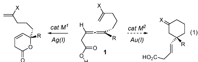
Figure 1. Allene templates for asymmetric annulation reactions.
