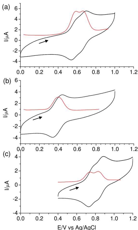
Figure 1. CV and DPV profiles of (a) 2^{2+} , (b) 4^{2+} , and (c) 7^{2+} in DMF containing 0.1 M \text{Bu}_4\text{NClO}_4 at a scan rate of 100 mV/s. DPV was measured with a step potential of 5 mV and an amplitude of 50 mV. The working electrode was glassy carbon, the counter electrode was a platinum wire, and the reference electrode was Ag/AgCl in saturated aqueous NaCl. For CV profiles with wider potential windows, see Figures S1–S3 in the Supporting Information.
