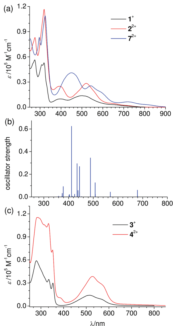
Figure 4. (a) Electronic absorption spectra of 1^{+} (black line), 2^{2+} (red line), and 7^{2+} (blue line) in acetonitrile. (b) TDDFT-predicted vertical excitations of 7^{2+} . (c) Electronic absorption spectra of 3^{+} (black line) and 4^{2+} (red line) in acetonitrile.
