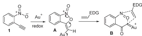
Scheme 1. Gold-Catalyzed Redox/Cycloaddition Cascade
