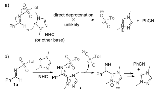
Scheme 2. Postulated pathways for the NHC-mediated generation of a sulfinic anion from an imine.
