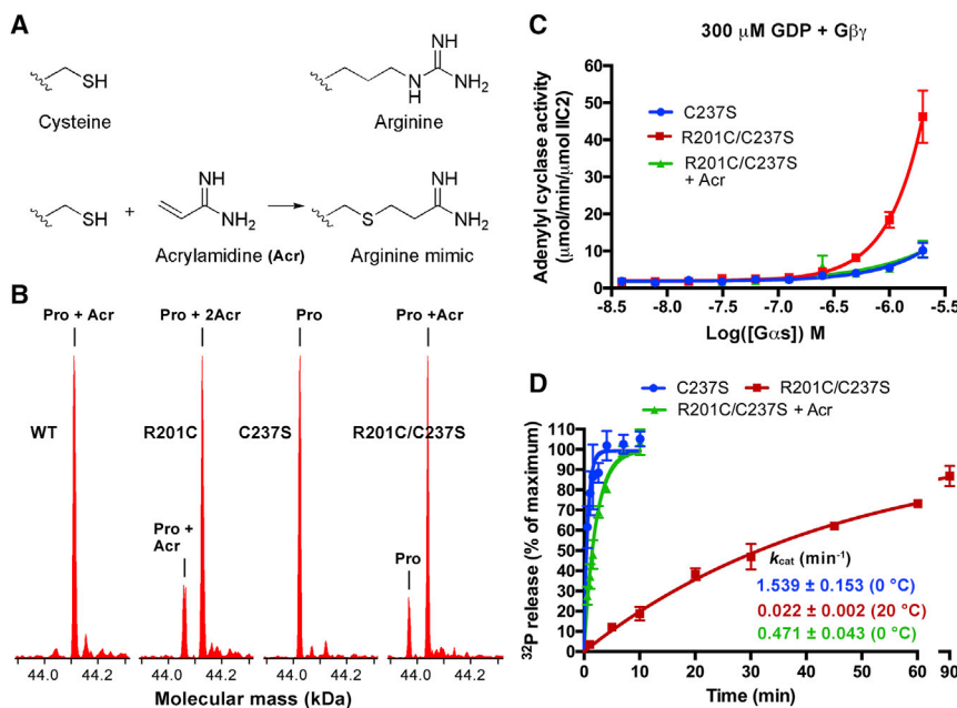
Figure 5. Modification of C201 by Acrylamidine Corrected the Adenylyl Cyclase-Activating Activity and Restored the Single Turnover GTPase Activity of the R201C Mutant (A) The structures of the side chain of cysteine and arginine, and the reaction between acrylamidine (Acr) and the side chain of cysteine. (B) Analysis of the modification of G\alpha_s using liquid chromatography and mass spectrometry (LC/MS). Before analysis, 6 \mu M G\alpha_s was incubated with 500 \mu M acrylamidine at room temperature for 2 hr. According to the molecular mass spectra, WT G\alpha_s was completely modified by one molecule of Acr, and mutating C237 to serine blocked this modification; introduction of the R201C mutation enabled G\alpha_s to be modified by one additional Acr. (C) Modification of C201 by acrylamidine decreased the adenylyl cyclase-activating activity of the R201C/C237S mutant. The adenylyl cyclase activity was measured in the presence of GDP and G\beta_1/\gamma_2 (C68S). The data represent the mean \pm SE of three independent measurements. (D) Modification of C201 by acrylamidine increased the single turnover GTPase activity of the R201C/C237S mutant to a level close to that of the C237S mutant. The data represent the mean \pm SD of at least three independent measurements.
