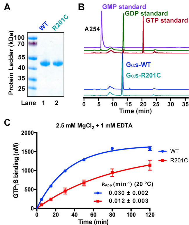
Figure S1. Nucleotide Occupancy and GTP \gamma S Binding Rates of WT G \alpha s and the R201C Mutant, Related to Figure 1
