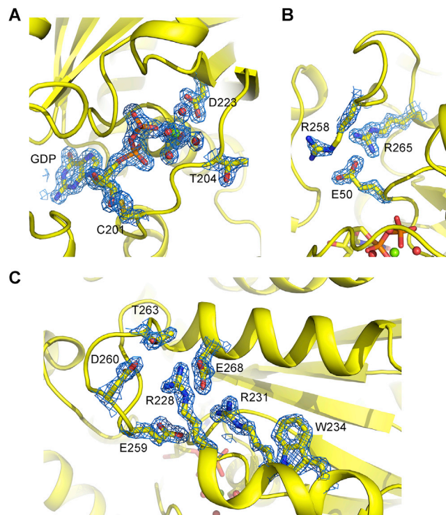
Figure S3. GDP and Water Molecules in the Nucleotide-Binding Pocket and Key Residues in the Hydrogen Bond Network of Gαs Are Well Defined in the 1.7 Å Structure of Gαs(R201C/C237S), Related to Figures 2 and 4
