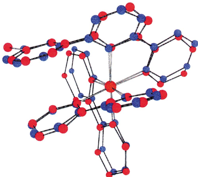
Fig. 5 Overlay of the structures of the [\text{Ru}(\text{bipy-}N,N')(\text{terpy-}N,N')]\text{PF}_6\text{PF}_6 (blue) and [\text{Ru}(\text{bipy-}N,N')(\text{bterpy-}N,N')]\text{PF}_6\text{PF}_6 (red) cations emphasising their similarity
