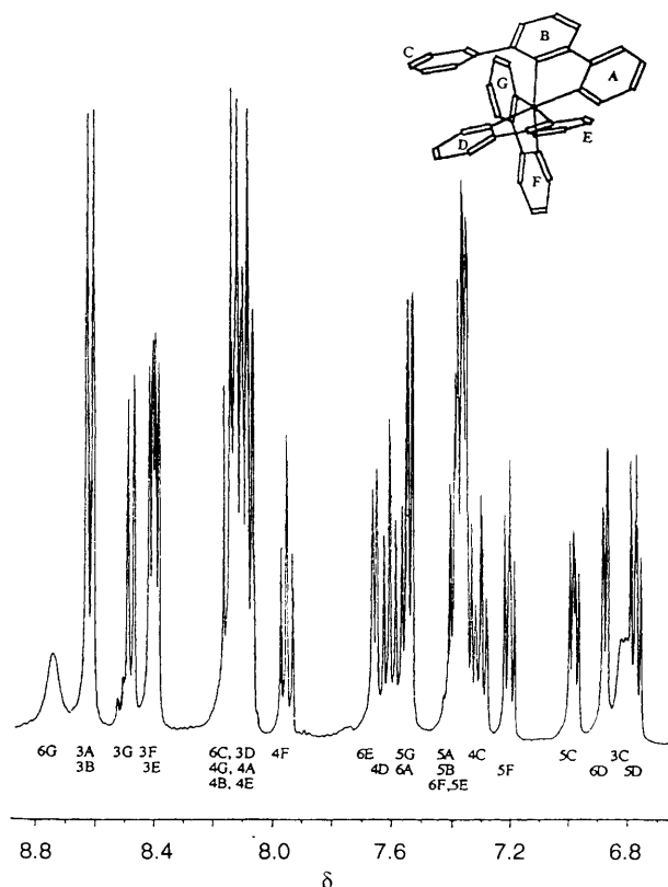
Fig. 6 The 400 MHz ^1\text{H} NMR spectrum of a \text{CD}_3\text{CN} solution of [\text{Ru}(\text{bipy-}N,N')(\text{terpy-}N,N')]\text{PF}_6\text{PF}_6 showing the assignments resulting from detailed two-dimensional studies
