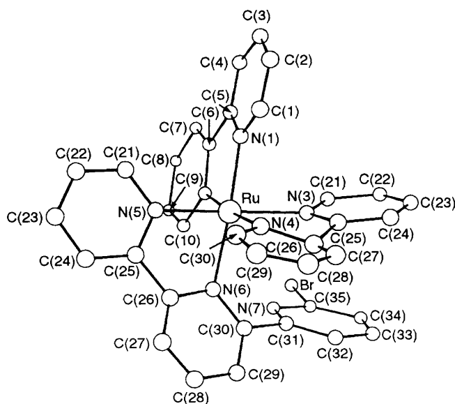
Fig. 4 Crystal and molecular structure of one of the enantiomers of the cation [\text{Ru}(\text{bipy-}N,N')(\text{bterpy-}N,N')]\text{PF}_6\text{PF}_6 showing the numbering scheme adopted. Hydrogen atoms have been omitted for clarity
