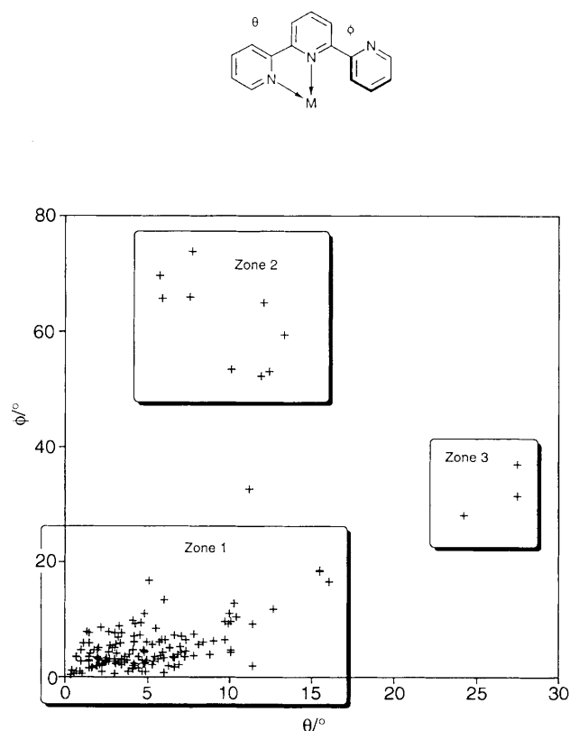
Fig. 2 Correlation of inter-ring dihedral angles for all metal 2,2':6',2''-terpyridine complexes found in the Cambridge Crystallographic Data Centre files
