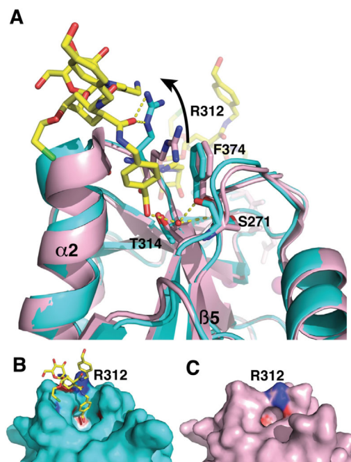
Figure 6. Non-canonical binding site of 16 . A) Overlay of DC-SIGN CRD X-ray structure (pink, PDB 1K9I) and DC-SIGN CRD co-crystallized with 16 (cyan, PDB 6GHV) highlighting the kink of helix-2 due to insertion of the p -hydroxymethylenebenzylamide fragment. A second copy of 16 in its canonical \text{Ca}^{2+} binding site can be seen in the back of the Figure, where the \text{Ca}^{2+} ion is shown in magenta. B) and C) The comparison between the two CRDs shows the cavity generated by Arg312 movement (see in A).
