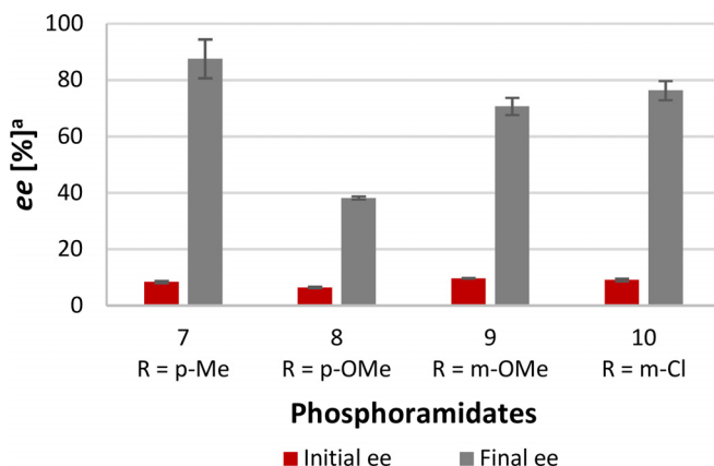
Figure 6. Chiral amplification results of phosphoramidate 7 , 8 , 9 and 10 in water at 26 °C. [a] Determined by chiral HPLC analysis.
