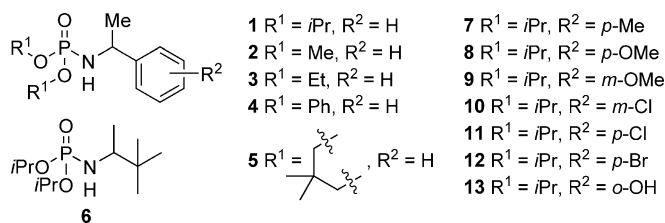
Figure 4. Phosphoramidates.
