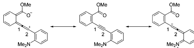
FIGURE 1. Carbomethoxy versus an N,N -dimethylamino group.
