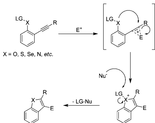
SCHEME 2. General Mechanism
