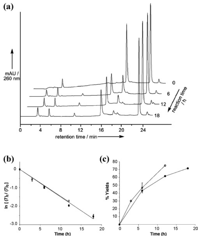
FIGURE 5. (a) HPLC analysis of the reaction mixture of the photolyzed duplex 5 and 3-amino-1,2-propanediol. The lactam 2b , the fragment 10-mer, 7 , and 9 eluted at 11, 16, 18, and 23 min, respectively. (b) Kinetics of the lactam formation from 7 in the single-stranded (○) and duplex forms (●) in phosphate buffer. Plots of \ln fraction substrate present versus time give k = 1.5 \times 10^{-1} \text{ h}^{-1} and t_{1/2} = 4.6 \text{ h} , respectively. (c) Yields of the lactam 2b from 5 in the single stranded (○) and duplex forms (●) in phosphate buffer.
