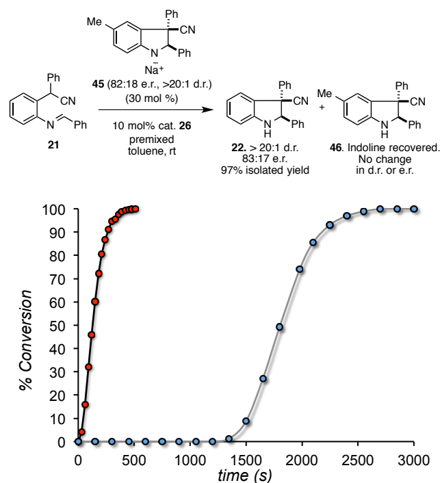
Figure 4: Plot of conversion to product versus time. Red markers indicate reaction progress in presence of preformed indolyl anion/ammonium salt mixture. T_0 corresponds to the time when the preformed indolyl anion/ammonium salt mixture was added to substrate. Blue markers are data from Figure 3 (for comparison).
