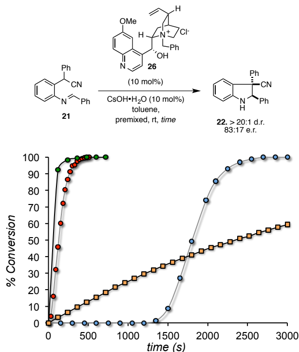
Figure 5: Plot of conversion to product versus time. Green circles indicate reaction progress after 6 h prestirring; orange squares indicate reaction progress after 30 mins prestirring. T_0 corresponds to the time when substrate was added to the reaction. Blue and red markers are data from Figures 3 & 4 respectively (for comparison).
