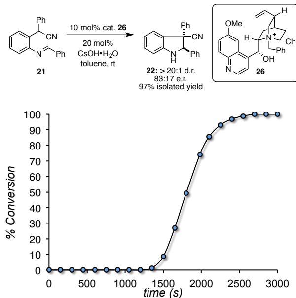
Figure 3: Plot of conversion to product versus time. T_0 corresponds to the time when base was added to the reaction mixture.
