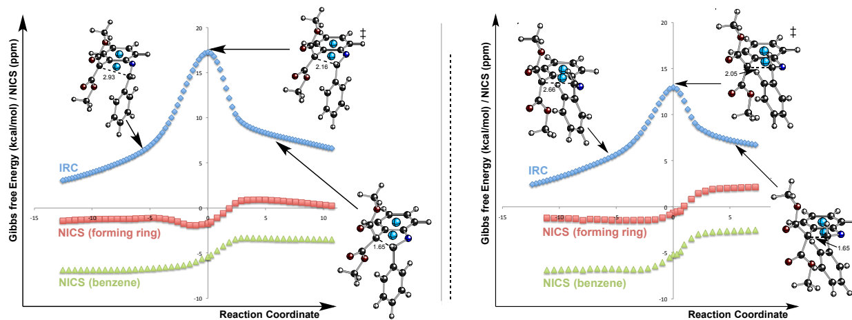
Figure 8: Intrinsic reaction coordinate (blue) and NICS values (red and green; blue spheres on structures indicate points at which NICS values were calculated) for ring-closure of Z- (left) and E- (right) imines; M06-2X/6-31+G(d,p) (forming C–C bond distances in Å).
