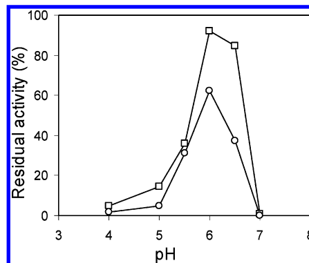
Figure 6. pH stability of \beta -galactosidase from L. reuteri L103 incubated at 37 °C in sodium citrate buffer (pH 4–5.5), sodium phosphate buffer (pH 6.0–7.5), and borate buffer (pH 8.0–9.0). The residual activity after 3 (□) and 20 h (○).
