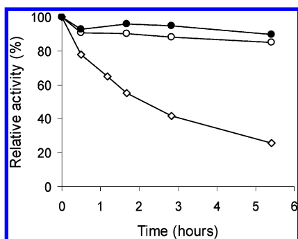
Figure 9. Stability of \beta -galactosidase from L. reuteri L461 at 42 °C without the presence of \text{MgCl}_2 (◇) and with the presence of 1 (O) and 10 mM (●) \text{MgCl}_2 . Experiments were performed in sodium phosphate buffer (pH 6.5).
