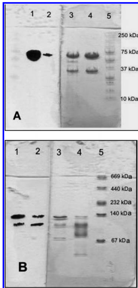
Figure 2. SDS-PAGE ( A ) and native PAGE ( B ) of purified \beta -galactosidases from L. reuteri L103 and L461. ( A ) Lanes 1 and 2 contained active staining with 4-methylumbelliferyl \beta -D-galactoside of \beta -galactosidases L461 (lane 1) and L103 (lane 2) and lanes 3–5 Coomassie blue staining of \beta -galactosidases L461 (lane 3) and L103 (lane 4) and recombinant molecular mass markers (Bio-Rad) (lane 5). ( B ) Lanes 1 and 2 contained active staining with 4-methylumbelliferyl \beta -D-galactoside of \beta -galactosidases L461 (lane 1) and L103 (lane 2), lane 3 \beta -galactosidase L461, lane 4 \beta -galactosidase L103, and lane 5 molecular mass markers (Amersham).
