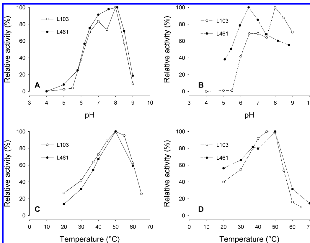
Figure 5. pH optimum (A and B) and temperature optimum (C and D) of \beta -galactosidases from L. reuteri L103 and L461 (A and C, o NPG as the substrate; B and D, lactose as the substrate).
