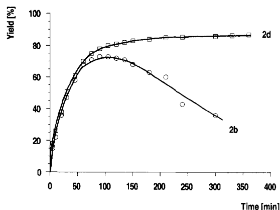
Fig. 2. Catalytic activity of \text{CH}_3\text{ReO} \cdot (\text{quinuclidine}) ( 2d ) (6 mol%) and \text{CH}_3\text{ReO} \cdot (\text{t-butylpyridine}) ( 2b ) (6 mol%) in the oxidation of cyclohexene with \text{H}_2\text{O}_2 . Cyclohexene: \text{H}_2\text{O}_2 : [\text{Cat.}] 1:1.5:0.01. T = 25^\circ\text{C} . If a ten-fold excess N -base: \text{CH}_3\text{ReO}_3 is used the resulting curve in both cases is identical with the curve for 2d within experimental error.
