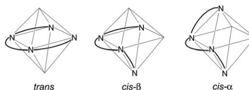
Figure 2. Stereoisomers of octahedral metal complexes.
