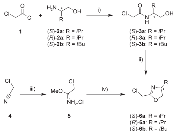
Scheme 1. Synthesis of 2-chloromethyl-2-oxazoline 6a and 6b . i) \text{NEt}_3 , \text{CH}_2\text{Cl}_2 , -20^\circ\text{C} , (83–89%); ii) Burgess reagent, THF, reflux, (51–66%); iii) \text{MeOH} , \text{Et}_2\text{O}\cdot\text{HCl} , (>95%); iv) amino alcohol 2 , \text{CH}_2\text{Cl}_2 , RT, (55–62%).
