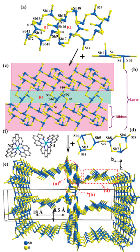
Figure 1. (a) 1D ribbon of [\text{Sb}_{10}\text{S}_{18}]_n^{6n-} . (b) trans - [\text{Sb}_2\text{S}_6] dimer. (c) [\text{Sb}_{12}\text{S}_{20}]_n^{4n-} layer. (d) [\text{Sb}_6\text{S}_{11}] unit. (e) 3D framework of 1 viewed along the a axis. (f) [\text{Ni}(\text{phen})_3]^{2+} cations in the channel.
