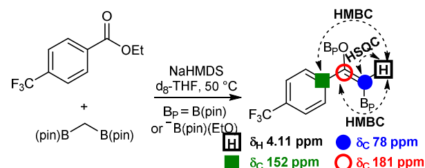
Scheme 5: Mechanism study
