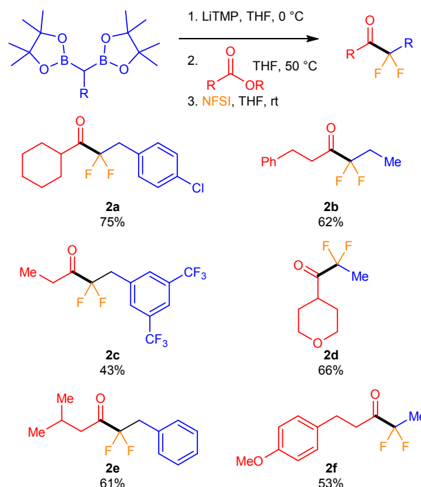
Scheme 3: Difluorinative coupling of enolizable esters
