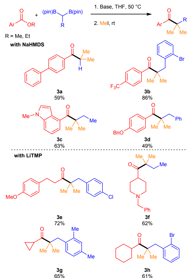
Scheme 4: Dimethylative coupling
