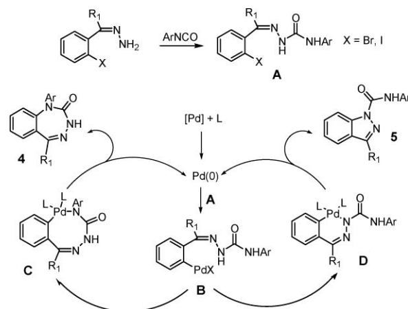
Scheme 3 Mechanistic hypothesis.
