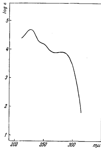
Fig. 1. Py-Tetrahydro-alstonin.
