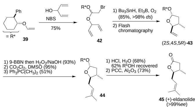
Scheme 6. Synthesis of (+)-eldanolide.
