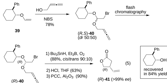
Scheme 5. Preparation of the enantiomerically enriched (>99% ee ) lactone ( R )- 41 .
