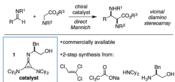
Figure 1. Vicinal diamino stereocenters via direct glycinate Mannich reaction.
