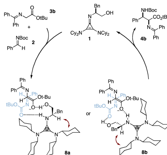
Figure 2. Proposed catalytic cycle for the cyclopropenimine-catalyzed Mannich reaction. The red double-headed arrow indicates conformational locking of the stereocenter due to steric conflict with a cyclohexyl ring.
