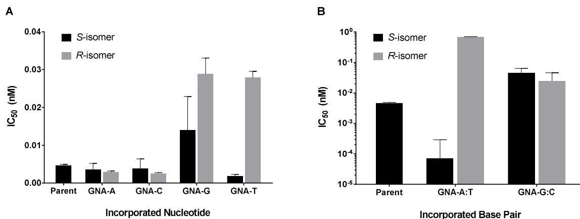
Figure 5. Effect of GNA incorporation on in vitro potency of unmodified siRNA targeting PTEN. Either a single nucleotide (panel A) or a single base pair (panel B) in the center of the duplex was substituted as indicated. See Supporting Information for sequence information.
