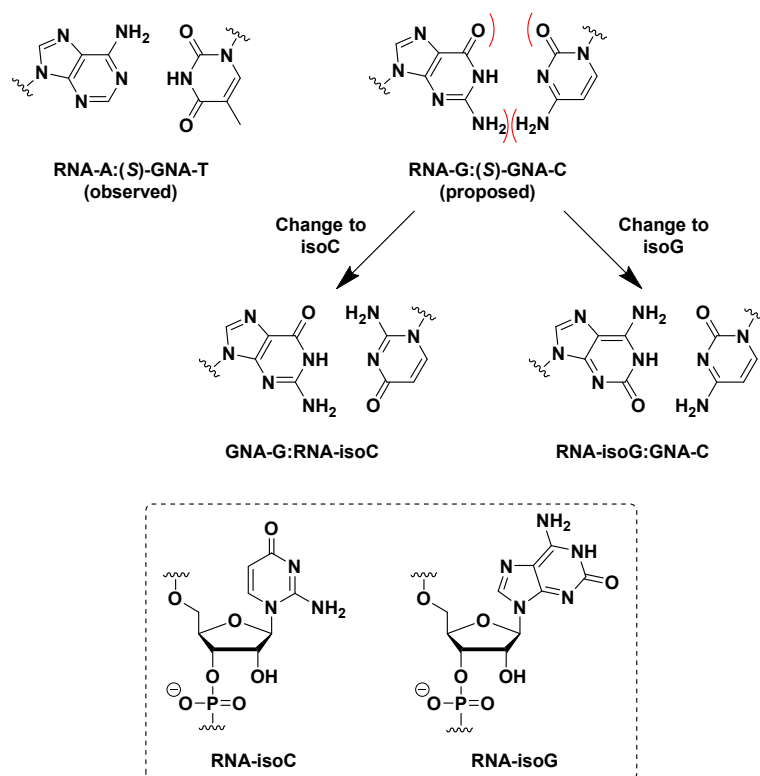
Figure 4. Structures of isocytidine and isoguanosine nucleotides and their potential to form fully complementary base pairs to “rotated” GNA-C or GNA-G.
