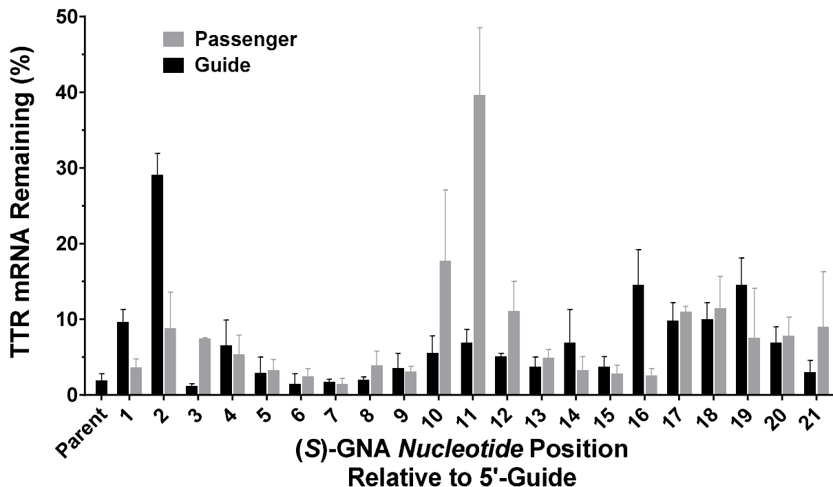
Figure 6. Positional impact of single ( S )-GNA nucleotide substitution on in vitro silencing activity at a concentration of 10 nM siRNA. The nucleotide at the indicated position of the guide or passenger strand was substituted with the corresponding GNA nucleotide. See Table S4 (Supporting Information) for sequence information.
