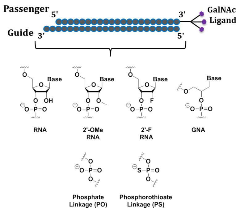
Figure 1. Structural overview of an siRNA-GalNAc conjugate duplex. 7 Also shown are the structures of the nucleotides used in this study, including 2'- O -methyl (2'-OMe), 2'-deoxy-2'-fluoro (2'-F), and GNA. Backbone modifications include both natural phosphate (PO) and phosphorothioate (PS) linkages.
