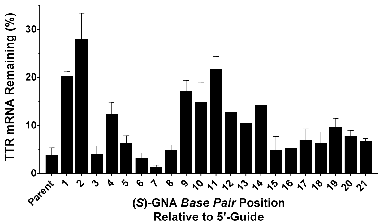
Figure 7. Positional impact of single (S)-GNA base pair substitution on in vitro silencing activity at a concentration of 10 nM siRNA. The base pair at the indicated position of the guide or passenger strand was substituted with the corresponding GNA base pair. See Table S4 (Supporting Information) for sequence information.
