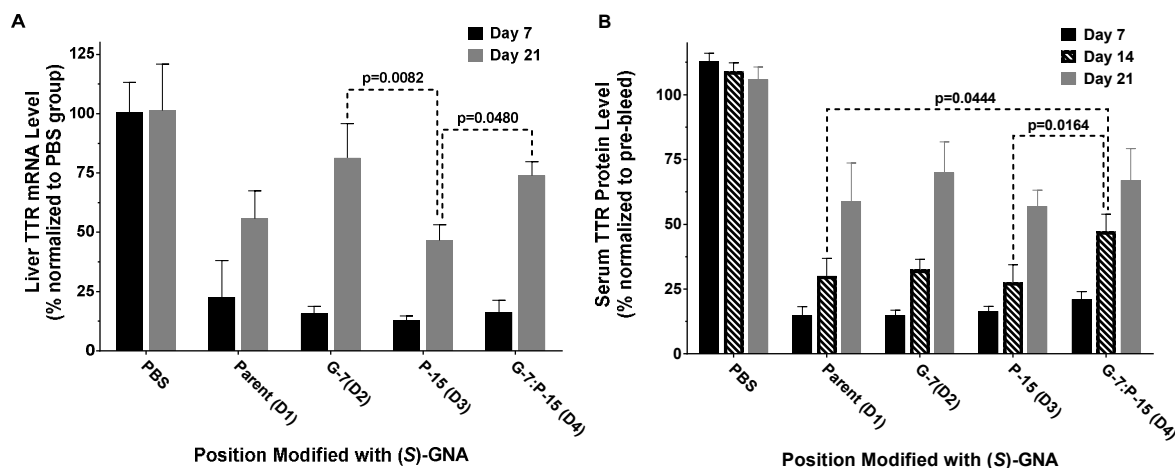
Figure 8. Knockdown of TTR in vivo with (S)-GNA modified siRNA duplexes dosed at 2.5 mg/kg. Error bars represent the SD from each cohort (n=3). Only those comparisons which are statistically significant are shown in the graph; all others are non-significant with the exception of all comparisons to PBS which were all significant. (A) TTR mRNA levels measured in the liver. (B) TTR protein levels measured in the serum. G = guide strand, P = Passenger strand.
