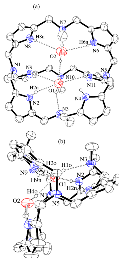
Figure 1. ORTEP diagram of hexapyrrolic pentaazacryptand 2a (30% thermal ellipsoids): (a) top view and (b) side view. Most hydrogen atoms are omitted for clarity. Selected bond lengths ( \text{\AA} ) and bond angles (deg): \text{N2}\cdots\text{O1} , 3.162(6) ; \text{H2n}\cdots\text{O1} , 2.36(3) ; \text{N2}-\text{H2n}\cdots\text{O1} , 162(5) ; \text{N8}\cdots\text{O2} , 3.236(8) ; \text{H8n}\cdots\text{O2} , 2.61(5) ; \text{N8}-\text{H8n}\cdots\text{O2} , 133(5) ; \text{N6}\cdots\text{O2} , 3.227(8) ; \text{H6n}\cdots\text{O2} , 2.51(4) ; \text{N6}-\text{H6n}\cdots\text{O2} , 146(4) .
