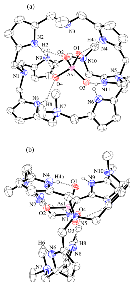
Figure 7. ORTEP diagram of the arsenate anion encapsulated complex 7 (30% thermal ellipsoids): (a) top view and (b) side view. Most hydrogen atoms are omitted for clarity. Selected bond lengths (Å) and bond angles (deg): As1–O1, 1.671(3); As1–O2, 1.700(4); As1–O3, 1.702(3); As1–O4, 1.664(3); O4–As1–O1, 113.40(17); O4–As1–O2, 107.32(18); O1–As1–O2, 109.03(18); O4–As1–O3, 107.41(14); O1–As1–O3, 110.10(17); O2–As1–O3, 109.49(16); C1–N1–C27, 111.1(3); C1–N1–C26, 110.2(3); C27–N1–C26, 110.0(3); C13–N5–C39, 111.5(3); C13–N5–C14, 111.1(3); C39–N5–C14, 109.7(3); C39–N5–N1–C1 = 45.94; C13–N5–N1–C26 = 46.69; C14–N5–N1–C27 = 47.66.
