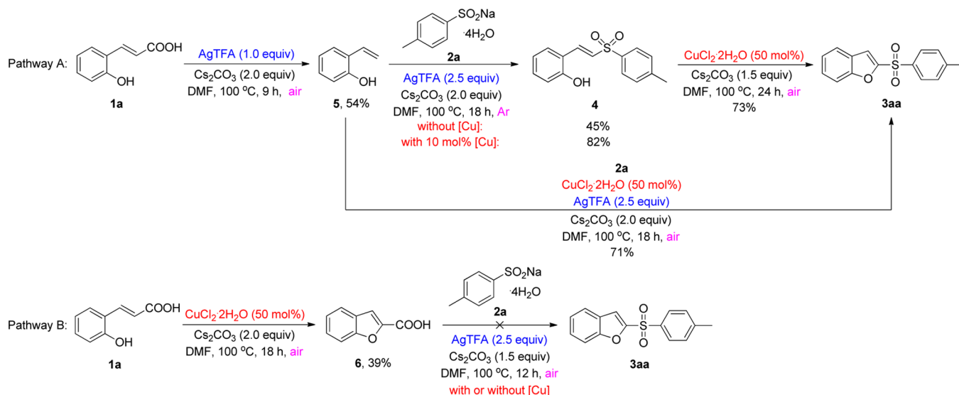
Scheme 4. Proposed Mechanism
