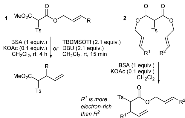
Scheme 1 dCr reactions of allylic 2-tosylmalonates.
