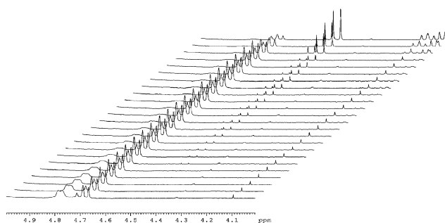
Fig. 2 1 H nmr spectra of dCr reaction of 1b recorded at 60 s intervals.
