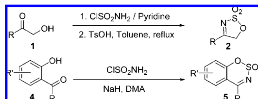
Scheme 2. Synthesis of Cyclic Activated Imines
