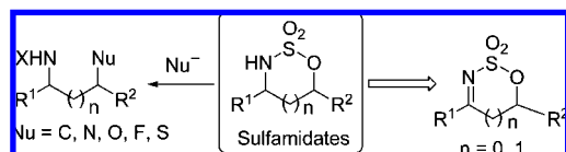
Scheme 1. Synthesis and Application of Sulfamides
