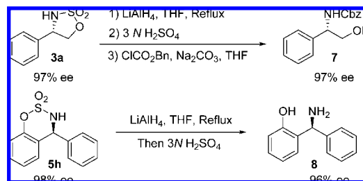
Scheme 4. Oxathiazinane Ring-Opening Reactions Using \text{LiAlH}_4
