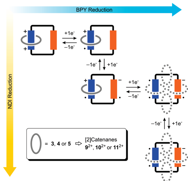
Figure 12. Co-conformational changes associated with the four reduction processes for [2]catenanes 9^{2+} – 11^{2+} . Horizontal and vertical processes represent the BPY-centered and NDI-centered reductions, respectively. The dotted gray ellipses indicate that the interactions are turned off and there is little information about the macrocycle location.
