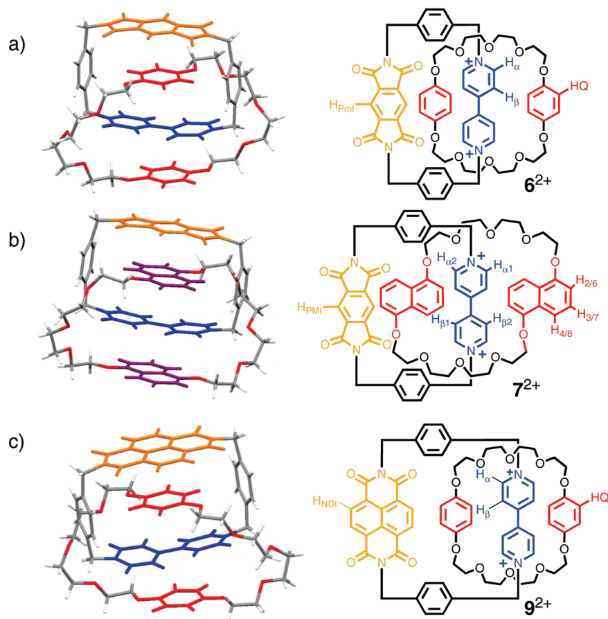
Figure 1. Stick representation of the solid-state structures and the structural formulas of (a) 6 •2PF 6 , (b) 7 •2PF 6 , and (c) 9 •2PF 6 . Solvent molecules and anions are omitted for clarity.
