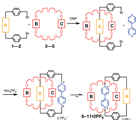
Scheme 1. Synthetic Scheme for the Desymmetrized [2]Catenanes
