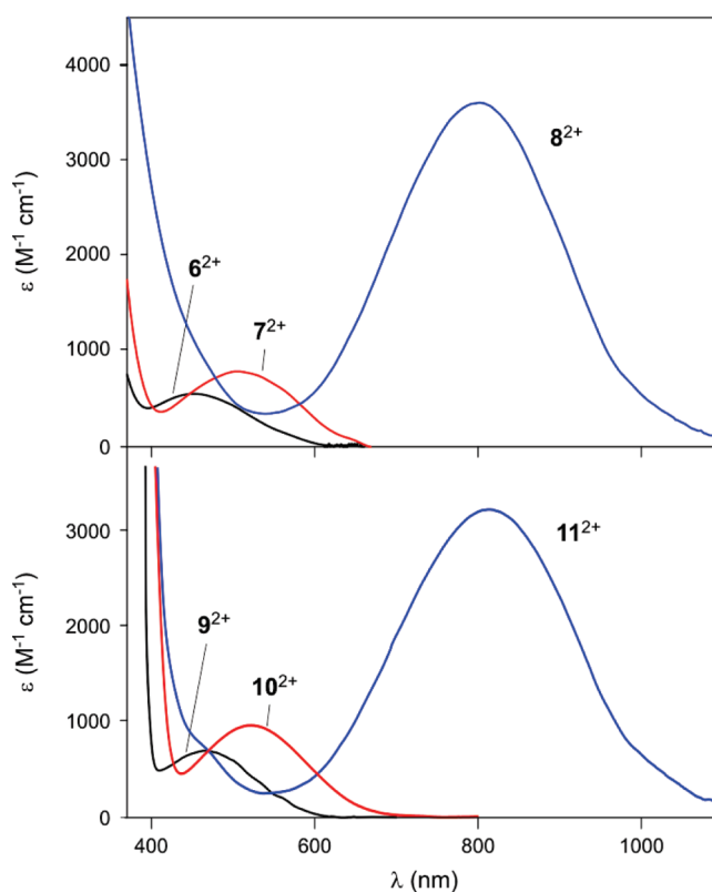
Figure 7. CT absorption bands of the [2]catenanes containing the PMI unit (top) and the NDI unit (bottom).
