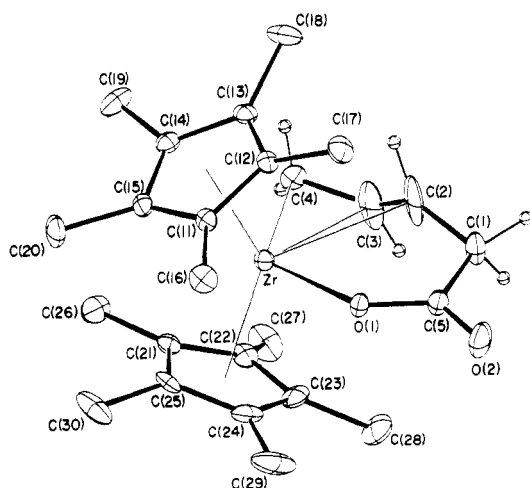
Figure 1. A perspective view of the \text{ZrCp}^*_2(s\text{-trans-C}_4\text{H}_6)/\text{CO}_2 (1:1) adduct (8). Thermal ellipsoids are drawn at the 20% probability level, and hydrogen atoms in \text{Cp}^* are omitted for clarity.
