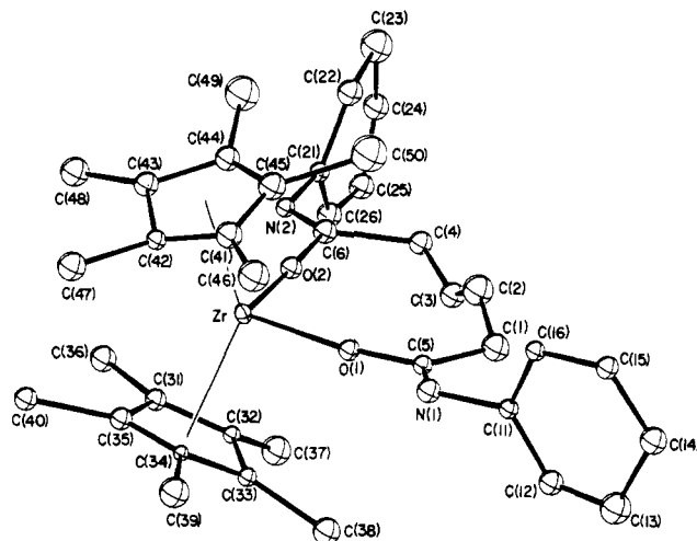
Figure 3. A perspective view of the \text{ZrCp}^*_2(s\text{-trans-C}_4\text{H}_6)/\text{C}_6\text{H}_5\text{NCO} (1:2) adduct ( 24a ) showing 10% probability thermal ellipsoids.
