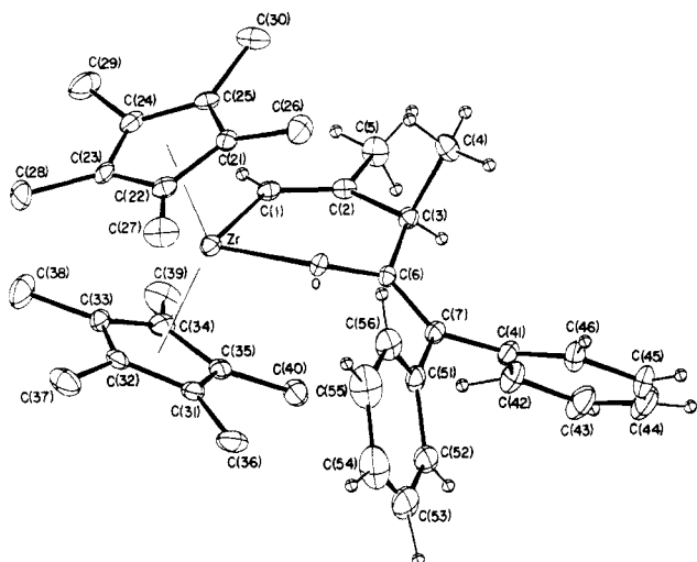
Figure 4. An ORTEP diagram of the \text{ZrCp}_2(s\text{-cis-isoprene})/\text{diphenylketene} (1:1) adduct ( 34 ). Thermal ellipsoids are drawn at the 20% probability level. Hydrogen atoms in \text{Cp}^* are omitted for clarity.
