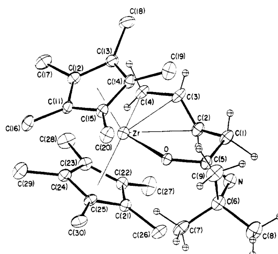
Figure 2. An ORTEP diagram and numbering scheme of the \text{ZrCp}^*_2(s\text{-trans-C}_4\text{H}_6)/t\text{-BuNCO} (1:1) adduct (23a) showing 20% probability thermal ellipsoids. Hydrogen atoms in \text{Cp}^* are omitted for clarity.
