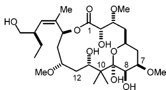
Figure 1. Peloruside A ( 1 ).
