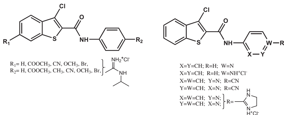
Fig. 1. Earlier prepared heteroaromatic benzo[b]thiophene-2-carboxamides.
