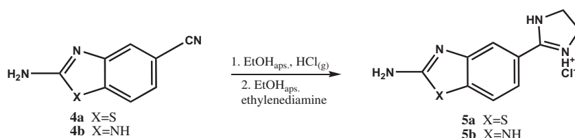
Scheme 3. Synthesis of 2-imidazolynyl substituted 2-aminobenzothiazole 5a and 2-aminobenzimidazole 5b .
