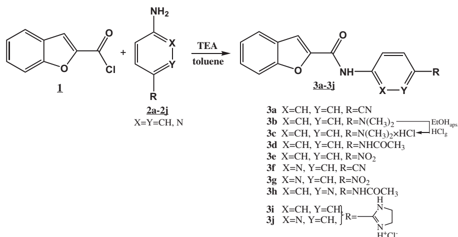
Scheme 1. Synthesis of benzofuran-2-carboxamide derivatives 3a–j .
