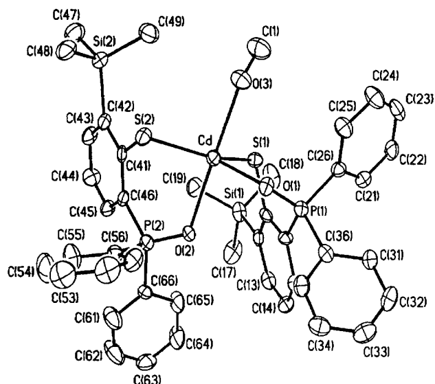
Figure 3. Molecular structure of [\text{Cd}\{2-(\text{Ph}_2\text{PO})-6-(\text{Me}_3\text{Si})\text{C}_6\text{H}_3\text{S}_2\}(\text{CH}_3\text{OH})] ( 3 ).
