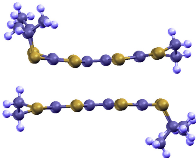
Figure 4. Packing of a pair of cations of 12 in crystal structure of \mathbf{12} \cdot \text{I}_3 .
