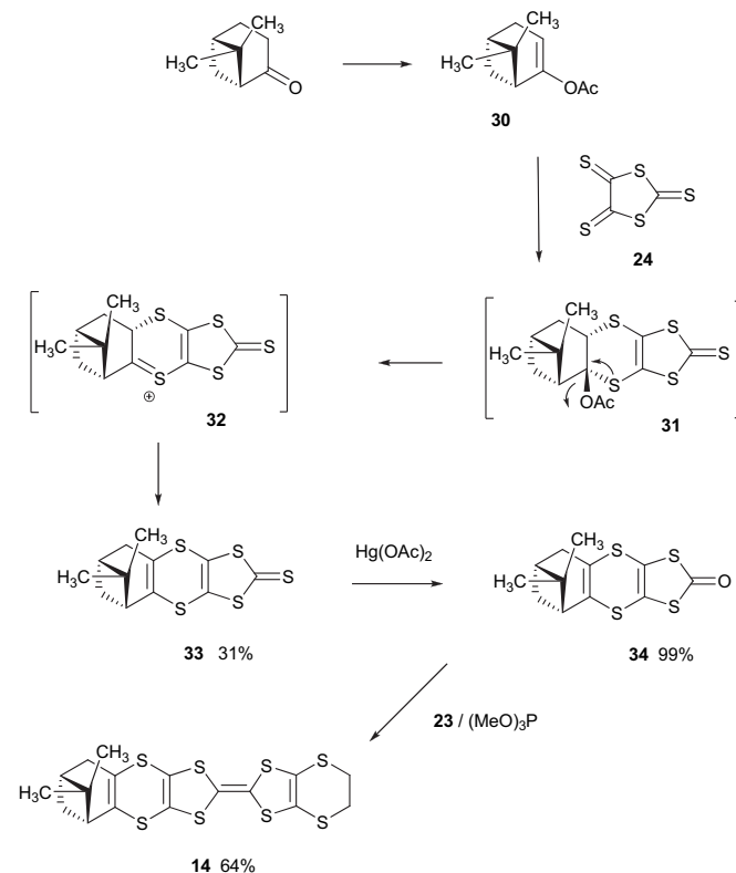
Scheme 4.
