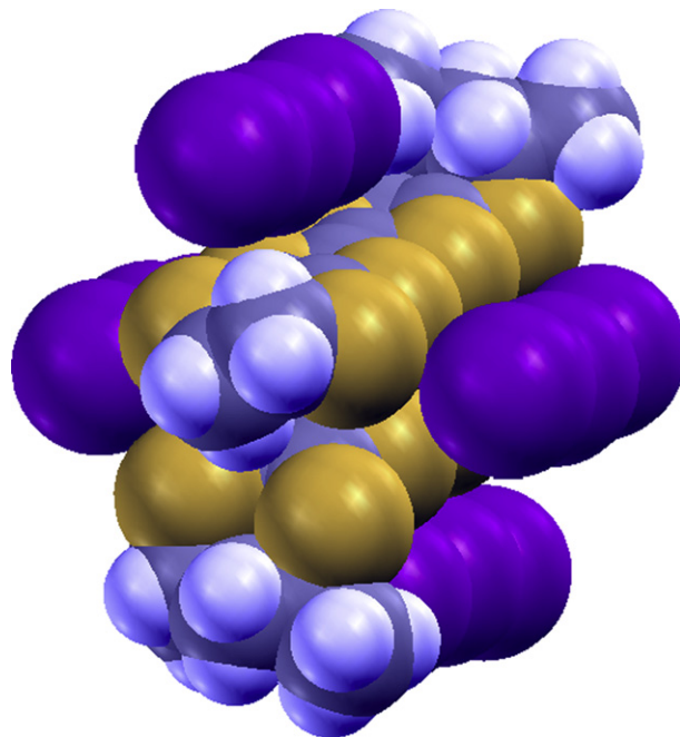
Figure 5. Local packing arrangement of cations of \mathbf{12}^+ surrounded by four triiodide ions.
