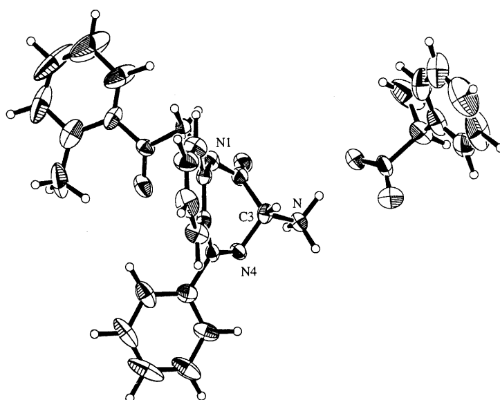
Fig. 2. An ORTEP Drawing of the Molecule of (R)- 25 (S)-Mandlate
