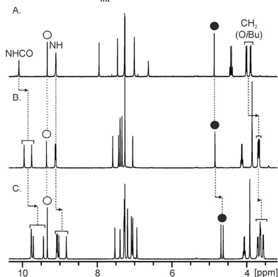
Figure 5. Part of the 300 MHz ^1\text{H} NMR spectra in \text{CDCl}_3 at 298K of: (A) tetramer 11 ; (B) nonamer 12 ; and (C) heptadecamer 13 . Signals of \text{H}_{\text{ext}} are marked with white circles. Signals of \text{H}_{\text{int}} are marked with full black circles.
