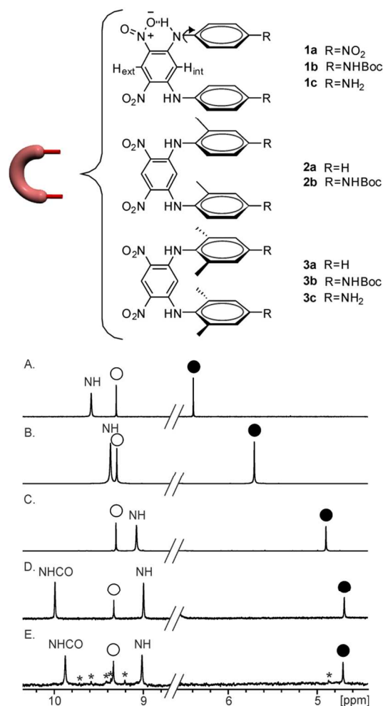
Figure 1. Part of the 300 MHz ^1\text{H} NMR spectra in \text{CDCl}_3 at 298K of: (A) hairpin turn in the phenyl series 1b ; (B) hairpin turn in the tolyl series 2b ; (C) hairpin turn in the xylyl series 3b ; (D) OiBu macrocycle 5a ; and (E) OMe macrocycle 5b . Signals of \text{H}_{\text{ext}} are marked with white circles. Signals of \text{H}_{\text{int}} are marked with full black circles. Stars indicate signals belonging to an impurity.
