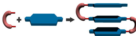
Chart 1. Study of the influence of substituents of adjacent rings on the folding of pseudo- \beta hairpins
