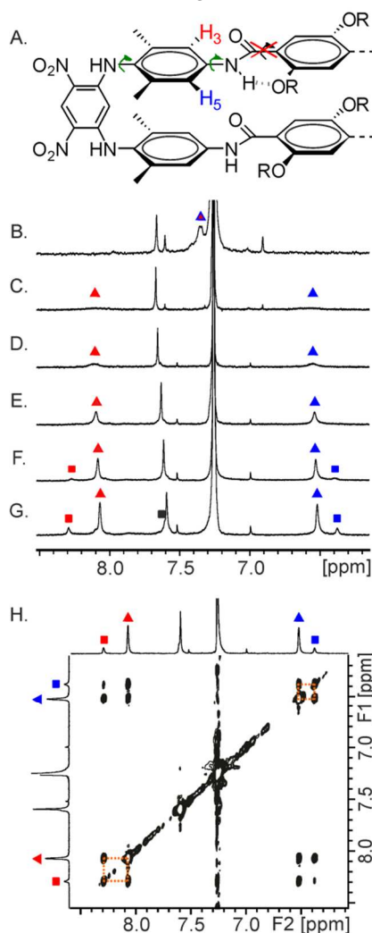
Figure 4. (A) Allowed rotations (green arrows) and rotation restricted by hydrogen bonding (red cross) of NH-aryl bonds in 5a and 5b . \text{H}_3 and \text{H}_5 are shown on the structure; Parts of the 400 MHz ^1\text{H} NMR spectra in \text{CDCl}_3 of: (B) 5b at 298 K; (C) 5a at 313 K; (D) 5a at 298 K; (E) 5a at 273 K; (F) 5a at 248 K; (G) 5a at 223 K. \text{H}_3 and \text{H}_5 signals are marked with red and blue triangles, respectively. \text{H}_3+\text{H}_5 fast exchange average signal is marked by a red-in-blue triangle. Signals belonging to a second conformer are marked with squares; (H) excerpt of the 2D ROESY plot ( \tau_m = 300 ms) at 223K showing chemical exchange between protons of the two conformers of macrocycle 5a .
