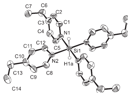
Figure 7. Structure of the dication [(4-Et-py) 4 SiH 2 ] 2+ in a crystal of 3e ·6CHCl 3 (ORTEP plot with 50% probability ellipsoids; C-bonded hydrogen atoms omitted for clarity). Selected bond lengths and bond angles are provided in Table 3.
