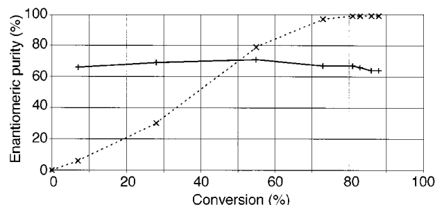
Fig. 1 Enantiomeric purity of (x) 1a and (+) 3a vs. conversion ¶ for the reaction of (±)- 1a with dimethyl 2-sodiummalonate catalysed by [\text{Ir(COD)Cl}]_2 –( R )- 6 .
