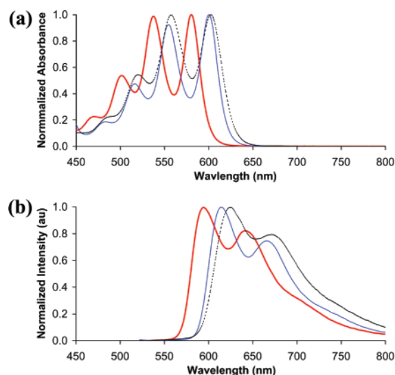
FIGURE 1. UV (a) and fluorescence emission (b) spectra of pentacenes 1a (bold red), 1b (blue), and 1c (dotted black) in dichloromethane at 120 \mu M and 6 \mu M, respectively. Fluorescence spectra were excited at 500 nm.
