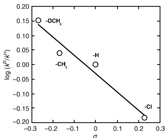
Fig. 5 Hammett plot for the oxygenation of [Cu(4'R-fla)_2] complexes (Table 8).
