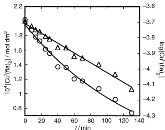
Fig. 4 Time course for the oxygenation of [Cu(fla)_2] in DMF (O) and plot of \log[Cu(fla)_2] ( \Delta ) versus reaction time for the oxygenation of [Cu(fla)_2] (experiment 5, Table 7).
