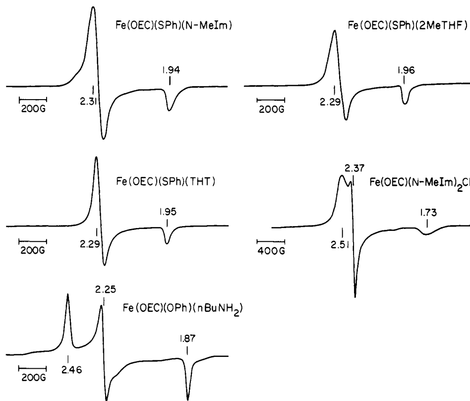
Figure 13. EPR spectra of selected low-spin \text{Fe}(\text{OEC})\text{LL}' species in toluene glasses at 80–85 K (g values are indicated).
