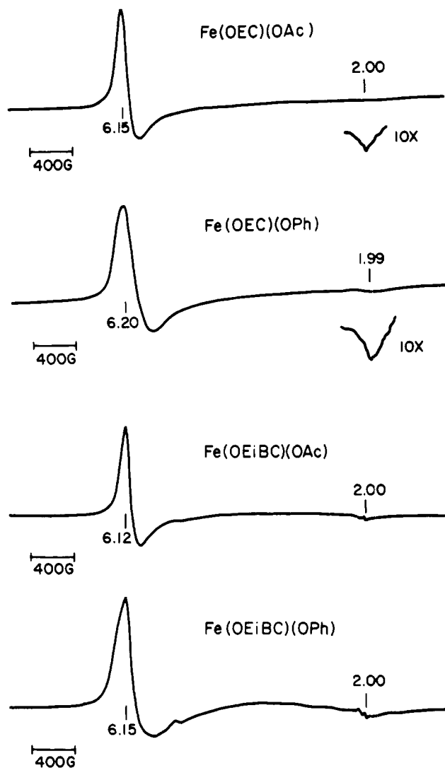
Figure 10. EPR spectra of high-spin hydroporphyrin Fe(P)L complexes ( L = \text{OAc}^- , \text{PhO}^- ) in toluene glasses at 80–85 K (apparent g values are indicated).
