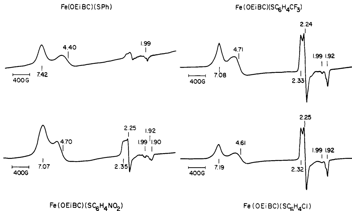
Figure 12. EPR spectra of mixtures of high-spin \text{Fe}(\text{OEiBC})(\text{SAr}) and low-spin \text{Fe}(\text{OEiBC})(\text{SAr})(\text{ArSSAr}) species in toluene glasses at 80–85 K (apparent g values are indicated).
