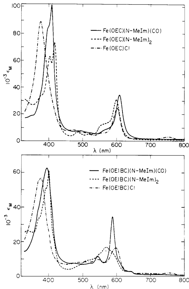
Figure 6. Absorption spectra demonstrating the conversion of Fe(P)Cl to Fe(P)(N-MeIm) 2 and the latter to Fe(P)(N-MeIm)(CO), reactions 5 and 6, in benzene solution at ambient temperature: upper, P = OEC; lower, P = OEiBC.
