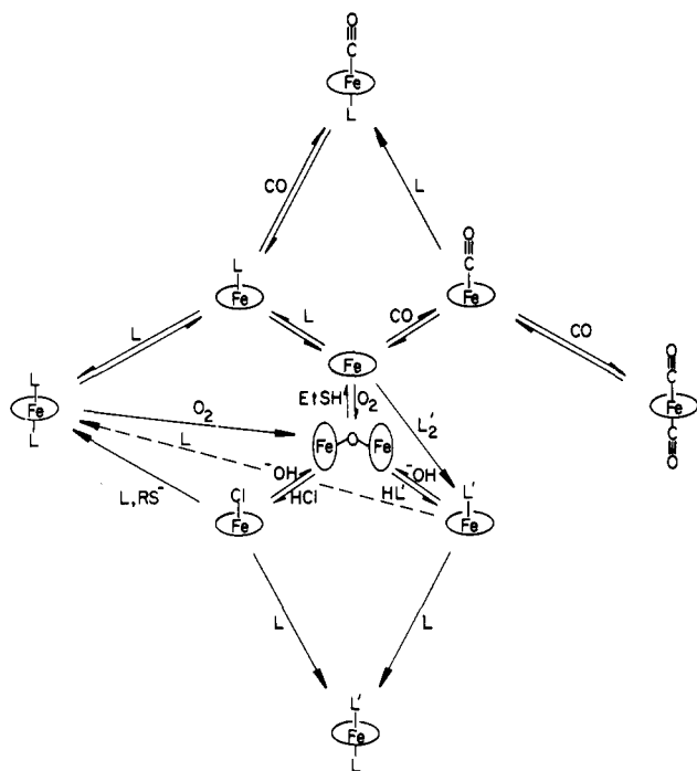
Figure 1. Generalized reaction scheme for \text{Fe}^{\text{II,III}}(\text{P}) complexes: \text{P} = \text{O} (OEP, OEC, OEiBC); \text{L} and \text{L}' are neutral or uninegative axial ligands. All species lying above and below the \mu -oxo-iron(III) complex contain \text{Fe}(\text{II}) and \text{Fe}(\text{III}) , respectively.
