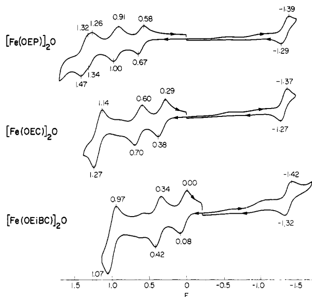
Figure 15. Cyclic voltammograms of [Fe(P)] 2 O complexes in dichloromethane solutions recorded at \sim 25^\circ\text{C} and 100 mV/s (peak potentials vs. SCE are indicated). The small waves preceding the major reductions presumably result from Fe(P)L species formed in cleavage of \mu -oxo complexes by acidic impurities in the solvent.
