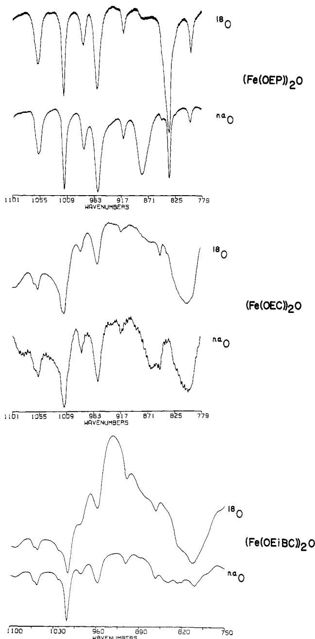
Figure 8. FT infrared spectra (1100–750 \text{cm}^{-1} ) of natural abundance ( ^{nat}\text{O} ) and ^{18}\text{O} -substituted [\text{Fe}(\text{P})]_2\text{O} complexes in paraffin oil mulls.
