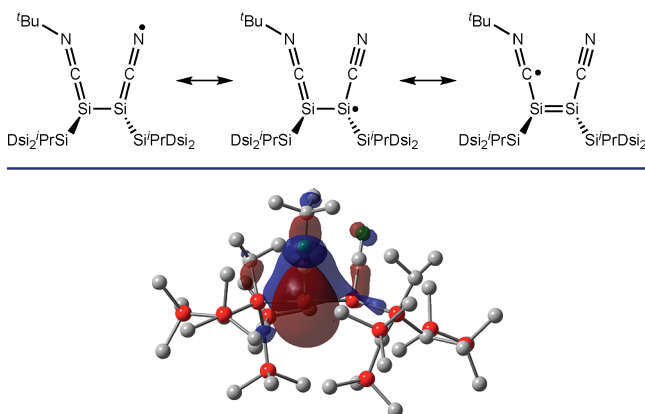
Figure 3. SOMO of [(Dsi 2 PrSi)SiSi(SiPrDsi 2 )(CN t Bu)(CN)] • at HF/6-31G(d).
