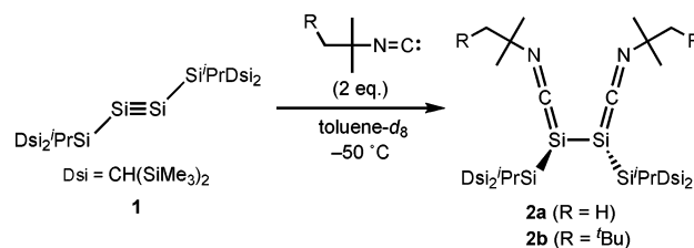
Scheme 1. Reaction of Disilyne 1 with tert -Butylisocyanide or tert -Octylisocyanide, Giving Disilyne–Isocyanide Adduct 2
