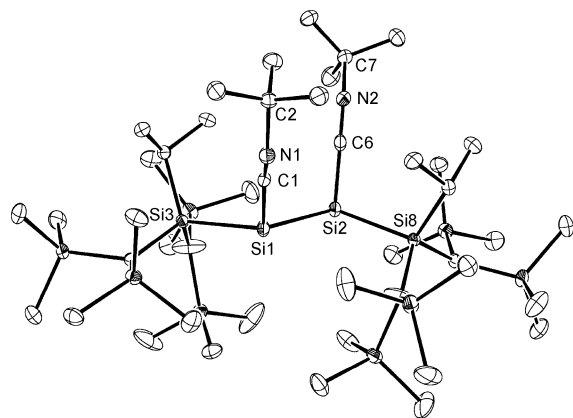
Figure 1. ORTEP drawing of 2a · \text{C}_5\text{H}_{12} (30% thermal ellipsoids). Hydrogen atoms and pentane molecule have been omitted for clarity. Selected bond lengths (Å) and angles (deg): Si1–Si2, 2.3575(17); Si1–Si3, 2.4070(16); Si1–C1, 1.809(4); Si2–Si8, 2.4220(16); Si2–C6, 1.803(5); N1–C1, 1.185(6); N1–C2, 1.476(5); N2–C6, 1.190(6); N2–C7, 1.485(6); Si2–Si1–Si3, 120.18(7); Si2–Si1–C1, 102.71(14); Si3–Si1–C1, 105.11(14); Si1–Si2–Si8, 114.65(7); Si1–Si2–C6, 104.36(15); Si8–Si2–C6, 103.90(14); C1–N1–C2, 144.0(4); C6–N2–C7, 143.5(4); Si1–C1–N1, 166.0(4); Si2–C6–N2, 176.5(4).
