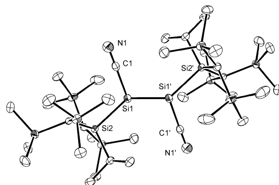
Figure 2. ORTEP drawing of 3 (50% thermal ellipsoids). Hydrogen atoms have been omitted for clarity. Selected bond lengths (Å) and angles (deg): Si1–Si1', 2.213(2); Si1–Si2, 2.3989(15); Si1–C1, 1.860(4); N1–C1, 1.120(4); Si1'–Si1–Si2, 136.48(9); Si1'–Si1–C1, 107.96(13); Si2–Si1–C1, 111.93(12); Si1–C1–N1, 178.6(4).
