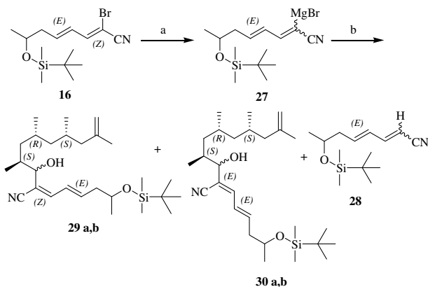
Scheme 5. Reagents and conditions: (a) i\text{-PrMgBr} , THF, -40^\circ\text{C} ; (b) 26 , THF, -40^\circ\text{C} , 28 (70%), 29ab (9%, 4%), 30ab (6%, 4%).
