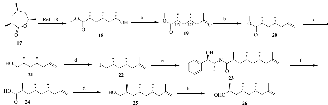
Scheme 4. Reagents and conditions: (a) \text{CrO}_3 , acetone, rt, 90%; (b) \text{PPh}_3\text{Br} , n\text{-BuLi} , THF, 0^\circ\text{C} , 66%; (c) \text{LiAlH}_4 , THF, rt, 1 h, 94%; (d) \text{PPh}_3 , \text{I}_2 , imidazole ACN/ether, rt, 2 h, 96%; (e) LDA, \text{LiCl} , (1 R ,2 R )-pseudoephedrine propionamide, rt, 18 h, 88%; (f) 2 N aq \text{NaOH}/t\text{-BuOH}/\text{MeOH} , reflux, 28 h, 91%; (g) \text{LiAlH}_4 , THF, rt, 1 h, 94%; (h) Dess–Martin periodanane, \text{CH}_2\text{Cl}_2 , rt, 76%.
